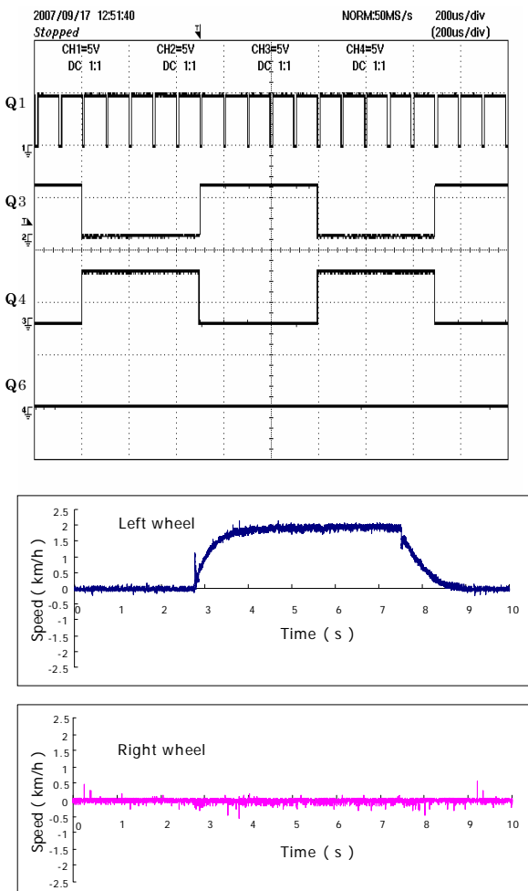
Fig. 15 Gate signals of MOSFETs and wheel speed (Switching duty ratio: Q_1=90\% , Q_6=0\% )
