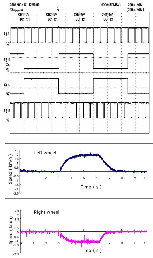
Fig. 16 Gate signals of MOSFETs and wheel speed (Switching duty ratio: Q_1=Q_6=90\% )
