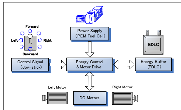
Fig. 3 Control system of the electric wheelchair
