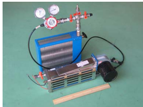
Fig. 2 PEM fuel cell and hydrogen storage alloys
