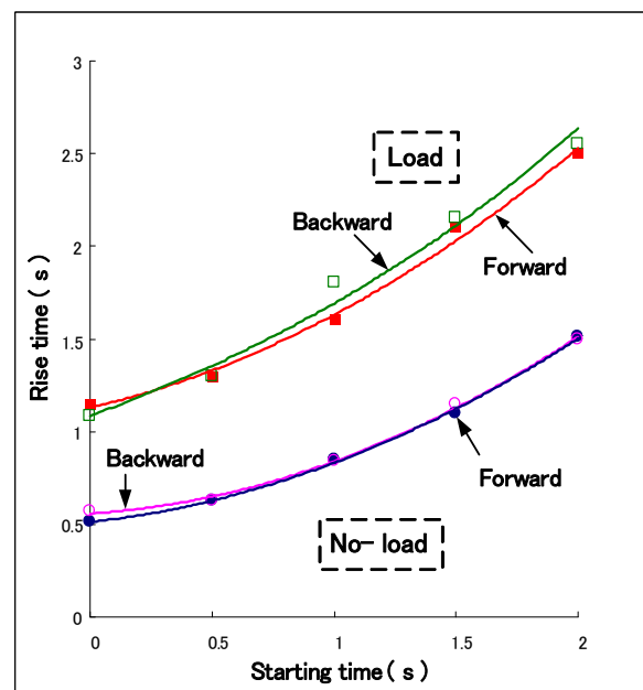
Fig. 14 Rise time to starting time
