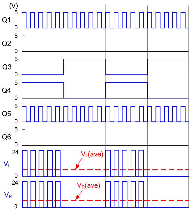
Fig. 10 Waveforms of the DC chopper (Forward)
