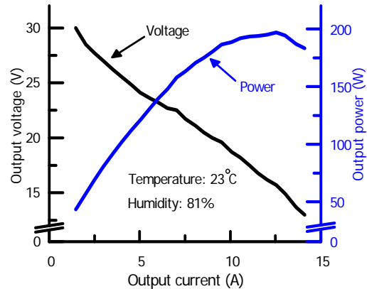
Fig. 6 Characteristics of the PEM fuel cell
