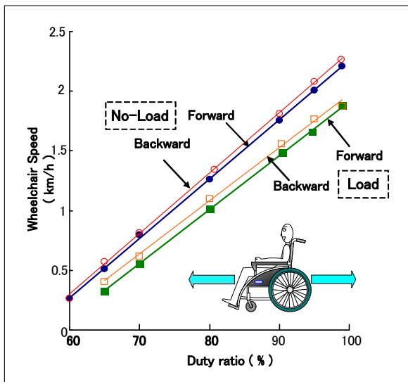
Fig. 11 Wheelchair speed to switching duty ratio
