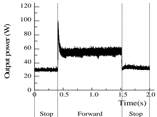
Fig. 7 Output power of the PEM fuel cell (Forward)
