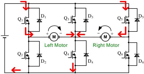
Fig. 9 Operation of the DC chopper (Forward)
